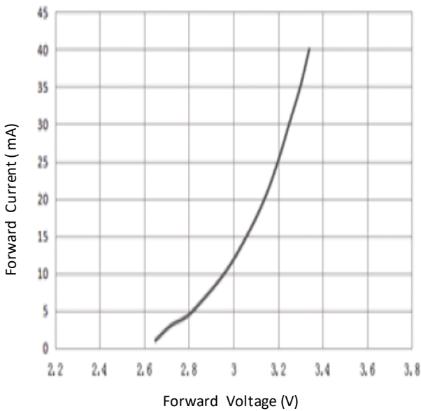
Fig. 3 Forward Current VS. Forward Voltage ( Ta=25C )
