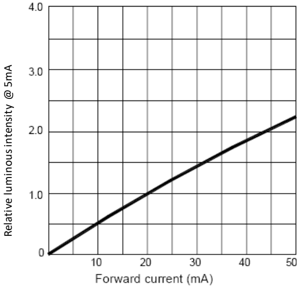
Fig 1. Relative luminous intensity vs Forward Current
