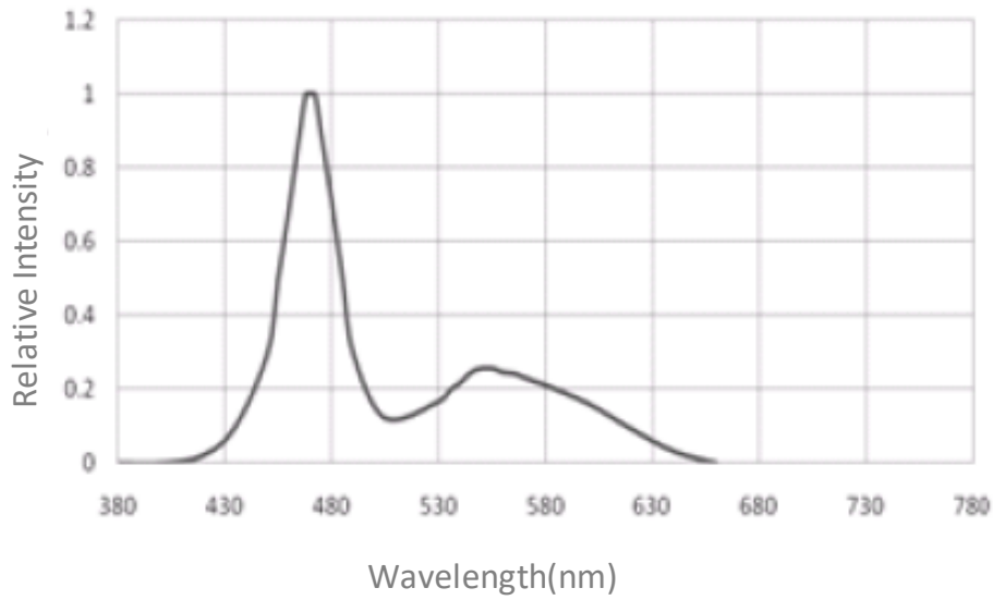
Fig 5. Spectrum Distribution (Ta=25°C)
