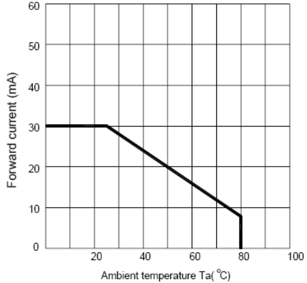
Fig.2 Forward current derating curve vs. ambient temperature
