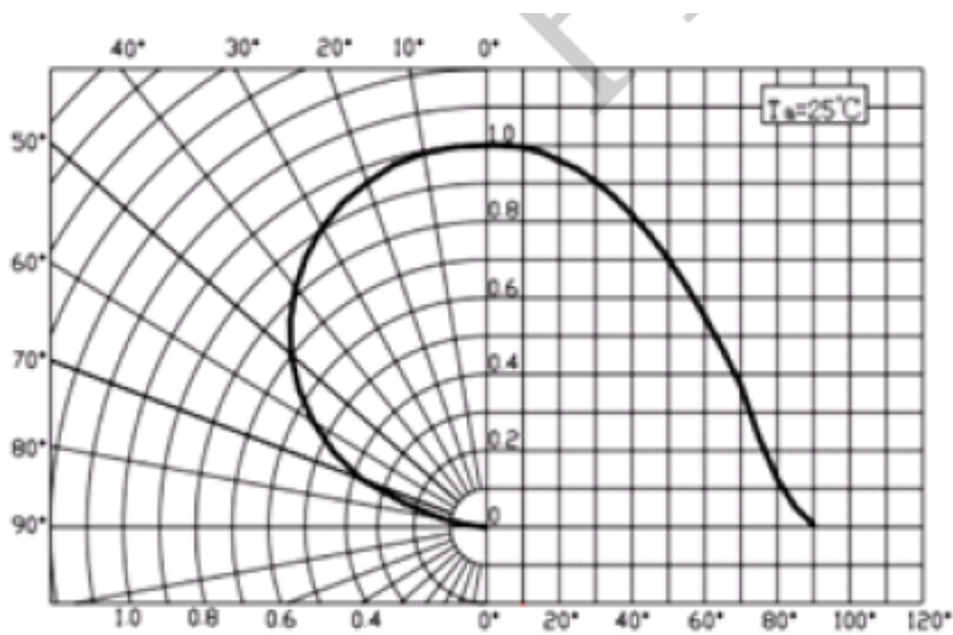
Fig.6 Radiation diagram
